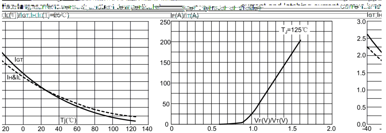
FIG 4: Relative variations of gate trigger current, holding
