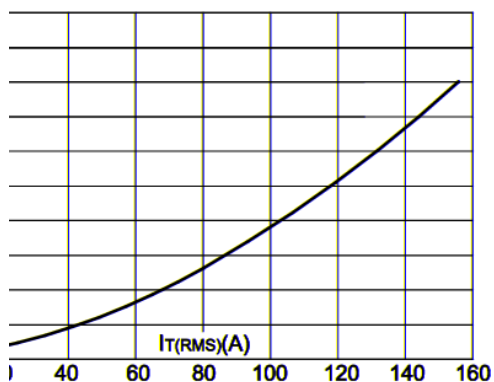
Power dissipation per module vs. R.M.S. current
