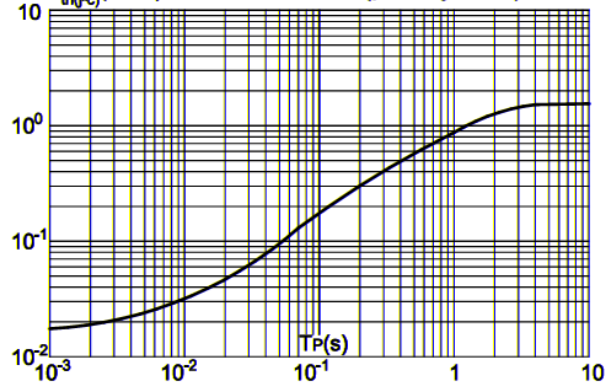
FIG.4: Maximum transient thermal impedance R_{th(j-c)}(^{\circ}C/W) Junction-to-case(per thyristor)
